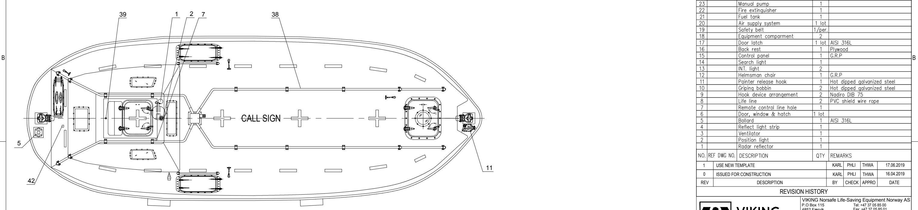
PLAN (BOAT ON PORT SIDE SHOWN)
